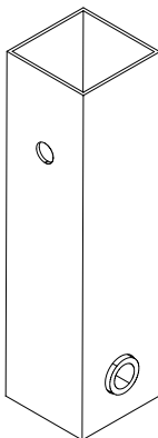
PART D RING PIN FRAME [ 1 PCS ]
