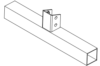
PART C LEFT LOWER FRAME [1 PCS]
